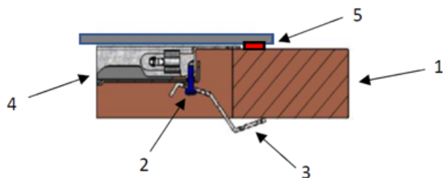
Attach the fastening clamps
